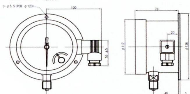
CGM-100-B 1接点
