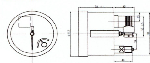
CGM-100-D 1接点
