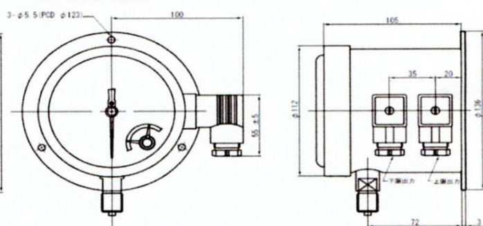
CGM-100-B 2接点
