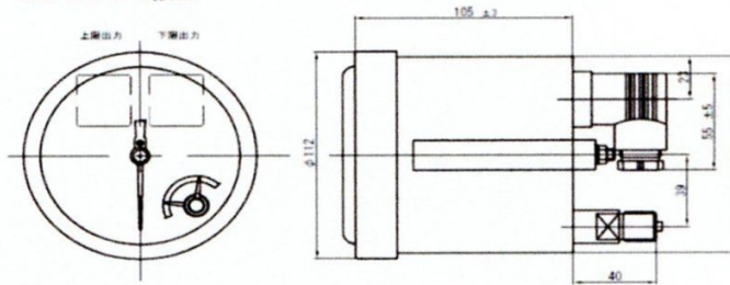
CGM-100-D 2接点
